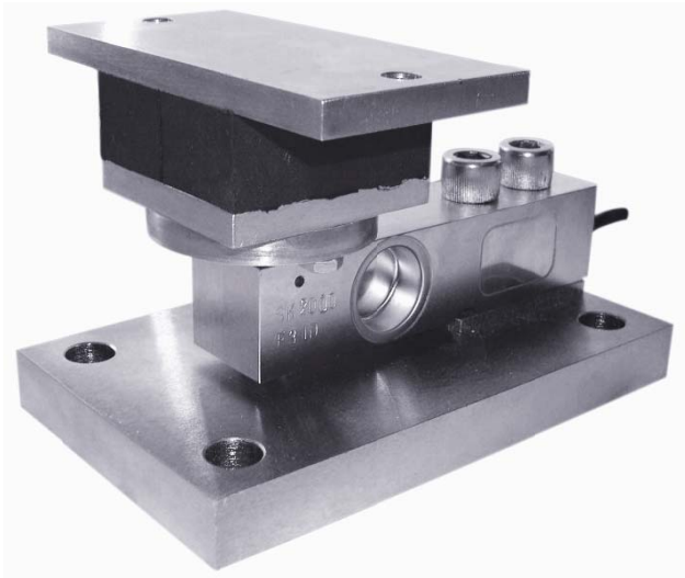
Scaime Iso Flex Rubber Mounting Assembly
